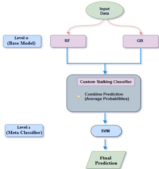
Fig. 5. Working procedure of proposed stacking ensemble model.
