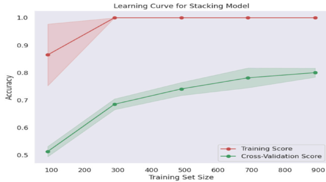
(i): Learning Curve for Stacking Ensemble Model
