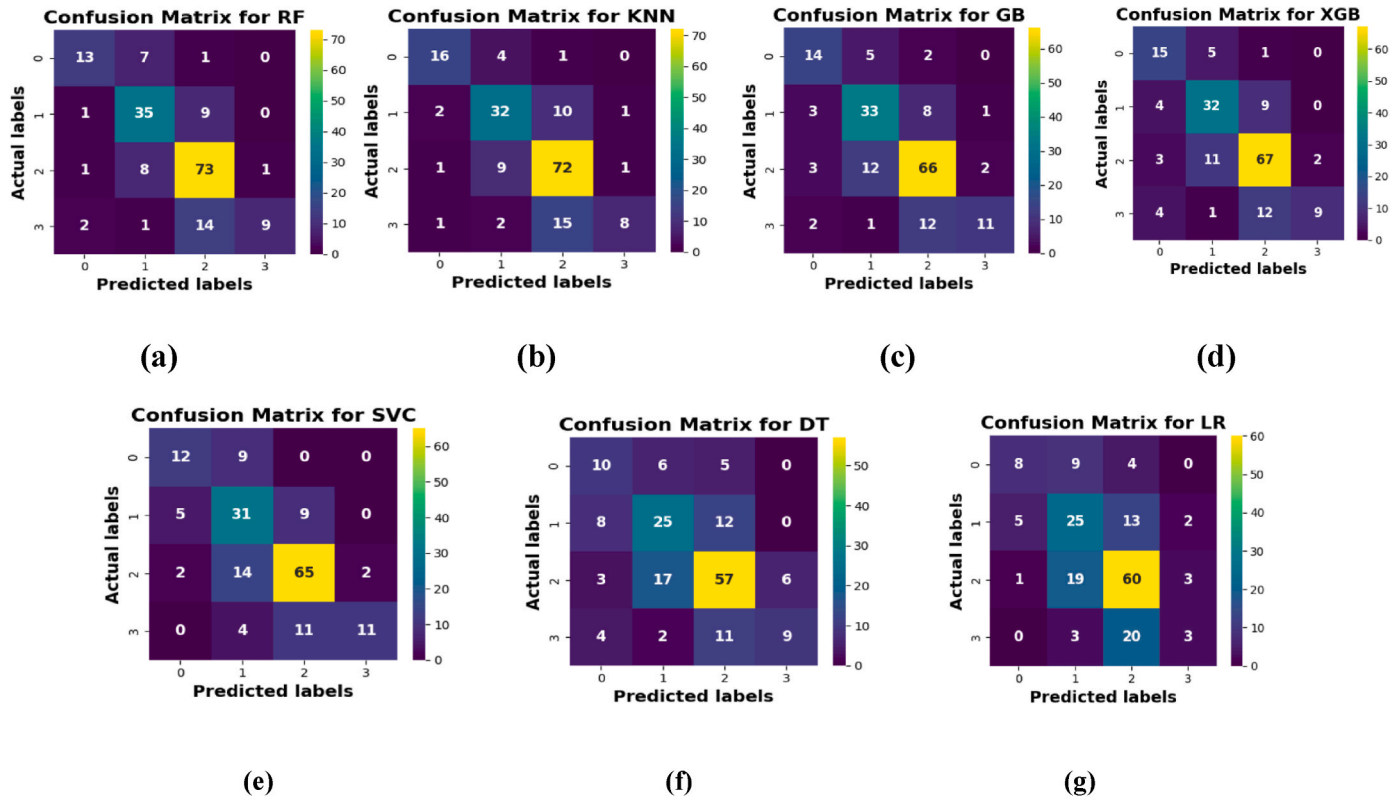
Fig. 6. 4x4 Confusion Matrix for ML classifier ((a)RF (b)KNN (c)GB (d)XGB (e)SVC (f)DT (g)LR) Before Applying Scaling Techniques.
