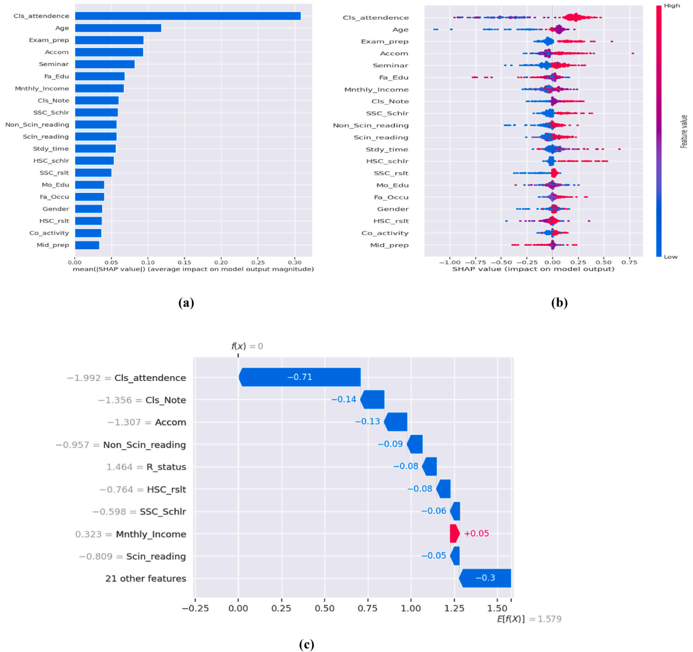
Fig. 10. (a) SHAP Value Counts for Each Feature; (b) Impact of SHAP Value on Model Output (Each class) (c) SHAP Waterfall Plot.
