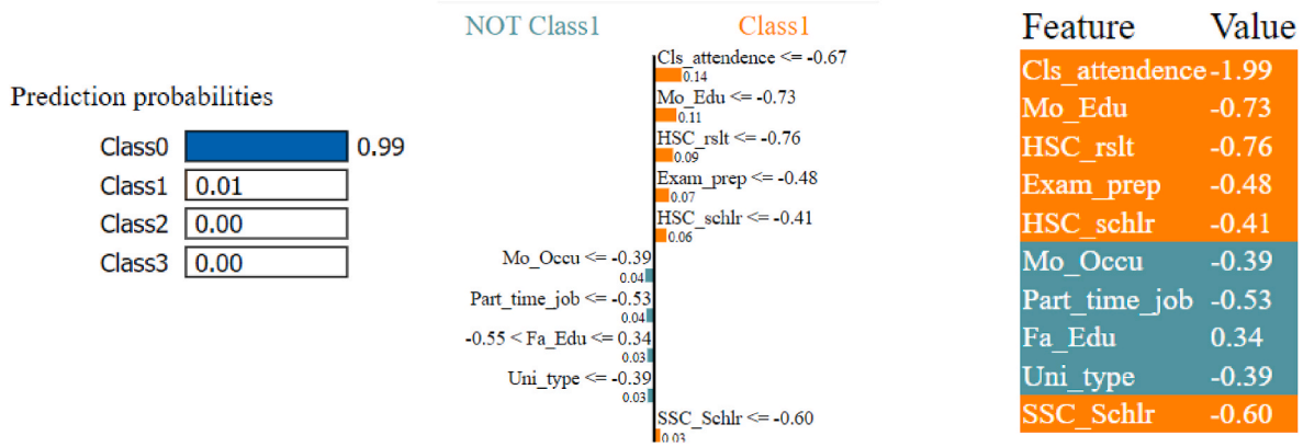
Fig. 12. Visualizing the stacking ensemble Model's output explanation (one instance) for LIME techniques.
