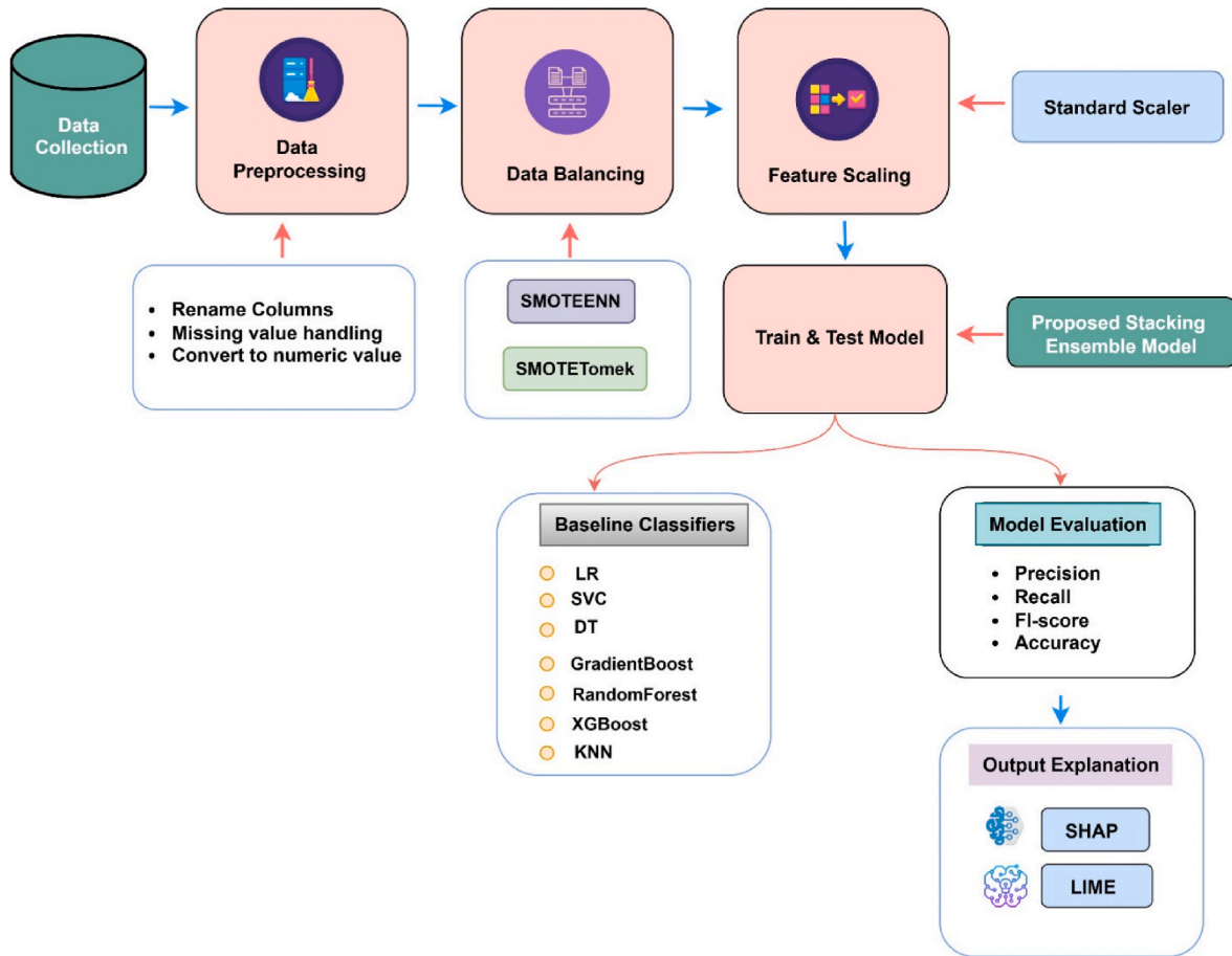
Fig. 1. Working Procedure of Student Performance Prediction using XAI.
