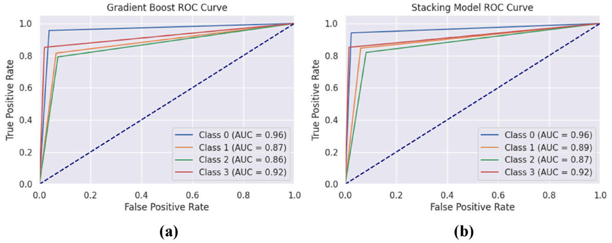
Fig. 9. Roc curve for (a) GB and (b) stacking ensemble model.
