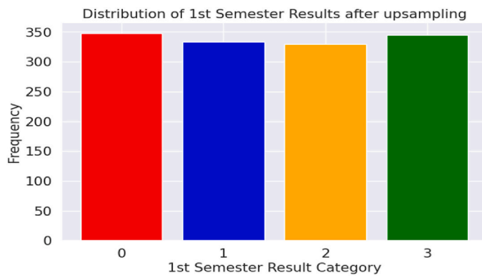
(a) Data balancing using SMOTETomek.
