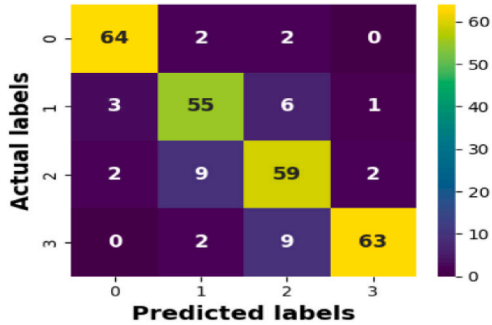
Confusion Matrix for Ensemble Model
